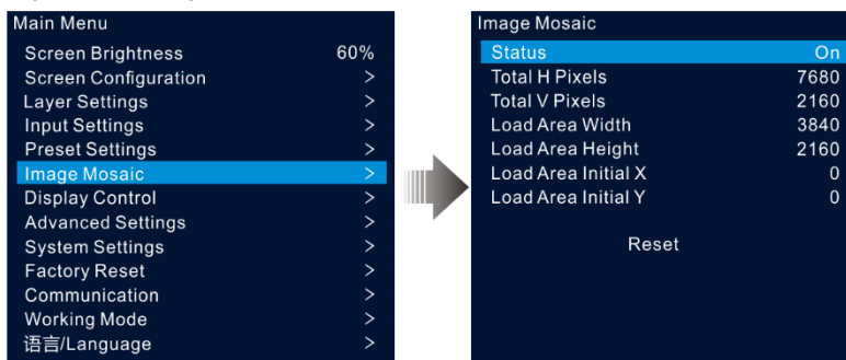
Figure 5-23 Image mosaic
