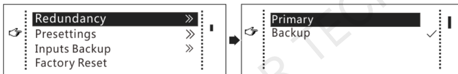
Figure 6-12 Redundancy settings
