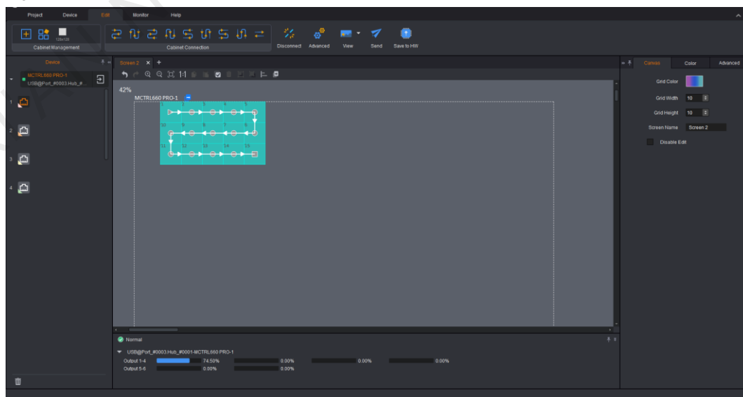
Figure 7-2 SmartLCT UI
