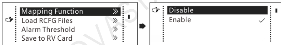
Figure 6-9 Mapping function
